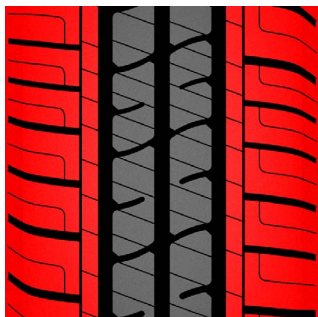
LARGE SHOULDER BLOCK WITH A NOISE-BLOCKING BAR. Reducing noise at the shoulder area delays premature wear and reduces sound that is generated by road traction.
