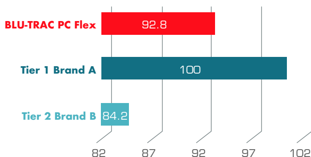
Ice Acceleration Index
